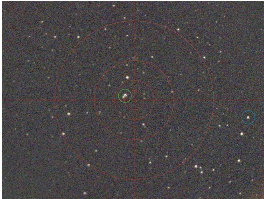
Figure 1: Photograph by Sanat Vidwans . WDS 21143+2522AB (green) and WDS 21139+2512 (blue), taken on July 29th at 22:01 PDT, 2022 near Big Finn Hill park, Kirkland, WA. The equipment used was a 130mm Newtonian reflector telescope with a 650mm focal length and a ZWO ASI224MC camera.
