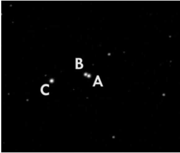
Figure 4. Sample Image of LEO 5 with Stars Labeled.
