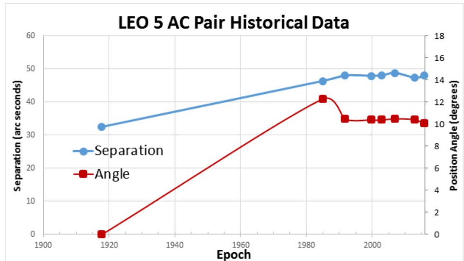
Figure 6. Graphical Representation of Historical Data Points for LEO 5 AC Pair.
